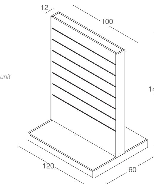
DGGD / L - N gondola dogata in nobilitato middle unit in faced panel L120 x P60 x H145 cm
