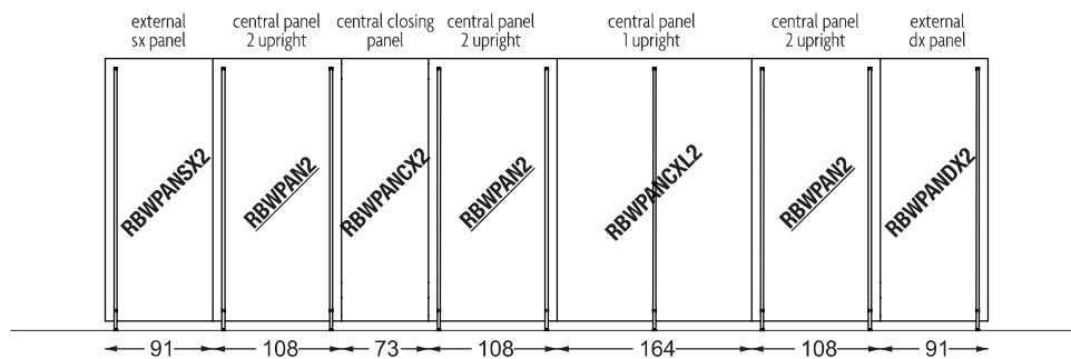
SCHEMA MONTANTI PASSO 90 DIAGRAM UPRIGHTS PITCH 90
