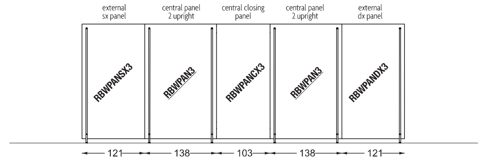
SCHEMA MONTANTI PASSO 120 DIAGRAM UPRIGHTS PITCH 120
